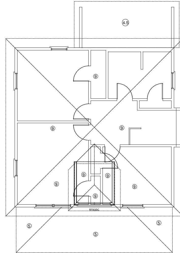
B 1 Roof Plan Scale: 1"=8ft. on B Sheet
