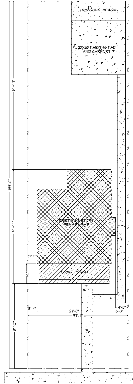
A 1 Site Plan Scale: 1"=20ft. on B Sheet
